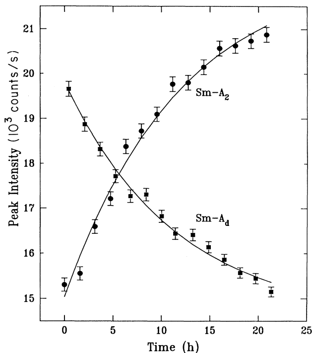
FIG. 11. Time dependence of the peak intensities at q_0=0.1206 \text{ \AA}^{-1} of the \text{Sm-A}_2 phase and q'=0.1336 \text{ \AA}^{-1} of the \text{Sm-A}_d phase (different vertical scales) at a fixed temperature ( 116.30^\circ\text{C} ) in the coexistence region after the sample is cooled from the \text{Sm-A}_d phase. The solid lines represent exponential fits both with the time constant of approximately 12.4 h.
