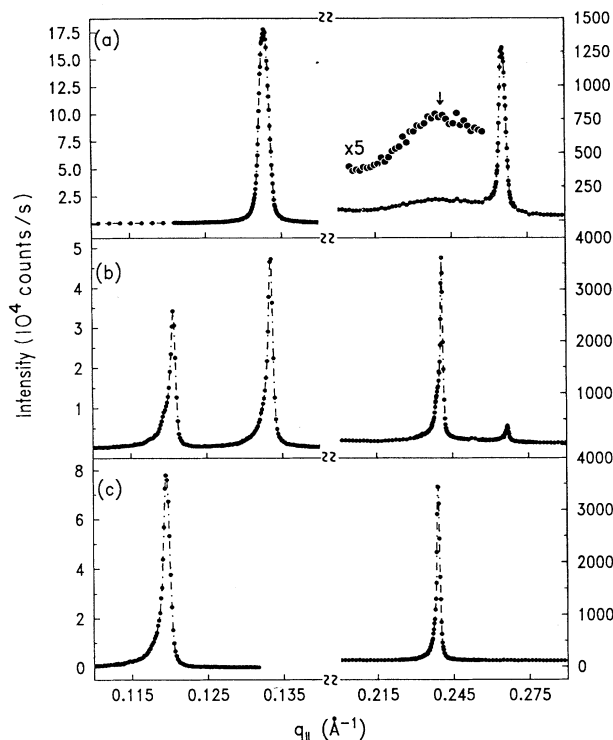
FIG. 8. Longitudinal ( q_{\parallel} ) scans taken at different temperatures for 35.1-mol% 8OCB in the 8OCB-plus-DB7OCN mixture. (a) In the \text{Sm-A}_d phase at 121.35^\circ\text{C} , there are two quasi-Bragg peaks at q' = 0.1328 \text{ \AA}^{-1} and 2q' = 0.2656 \text{ \AA}^{-1} , and a diffuse peak (also shown on 5\times scale) at 2q_0 \sim 0.2389 \text{ \AA}^{-1} . (b) In the coexistence region at 115.69^\circ\text{C} , two \text{Sm-A}_d peaks at q' = 0.1335 \text{ \AA}^{-1} and 2q' = 0.2667 \text{ \AA}^{-1} , and two \text{Sm-A}_2 peaks at q_0 = 0.1206 \text{ \AA}^{-1} and 2q_0 = 0.2409 \text{ \AA}^{-1} are simultaneously present. (c) At 105.22^\circ\text{C} , only two \text{Sm-A}_2 peaks at q_0 = 0.1196 \text{ \AA}^{-1} and 2q_0 = 0.2390 \text{ \AA}^{-1} remain.
