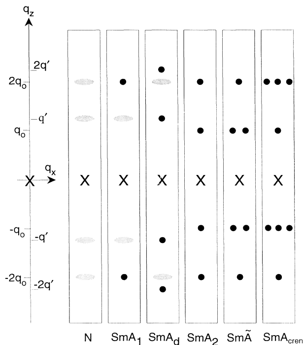
FIG. 2. X-ray-diffraction patterns for the phases exhibited by polar liquid crystals. The solid dots represent quasi-Bragg peaks from smectic structure and the shaded ellipses represent diffuse scattering due to short-range (liquidlike) molecular arrangement. Here, q_z is along the smectic layer normal. The wave number 2q_0 = 2\pi/l , l being the molecular length, corresponds to the monolayer ( \text{Sm-A}_1 ) phase while q' = 2\pi/2l' corresponds to the partial bilayer ( \text{Sm-A}_d ) phase. Note that the \text{Sm-}\tilde{A} and \text{Sm-A}_{\text{cren}} phases have quasi-Bragg reflections with nonzero value of transverse component ( q_x ) of the scattering vector.
