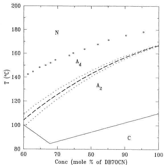
FIG. 17. The phase diagram of the 8OCB-plus-DB7OCN system replotted with the DB7OCN concentration along the abscissa. The dotted curves approximately define the boundaries of the Sm- A_d to Sm- A_2 coexistence and the dashed line in this region represents the first-order Sm- A_d to Sm- A_2 transition.
