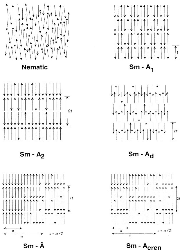
FIG. 1. Schematic representations of the polar nematic and smectic- A phases. The molecules are drawn as thin rods with arrows on one end to denote the longitudinal dipoles. Here, l is the molecular length and 2l' ( l < 2l' < 2l ) is the effective length of dimerlike molecular arrangements formed in the \text{Sm-A}_d phase. The smectic layer spacings of various phases are shown in terms of l and l' . In the \text{Sm-}\tilde{A} and \text{Sm-A}_{\text{cren}} phases, the in-plane modulation has the repeat distance m . In these phases a and (m - a) represent the widths of adjacent antiphase regions as discussed in the text.
