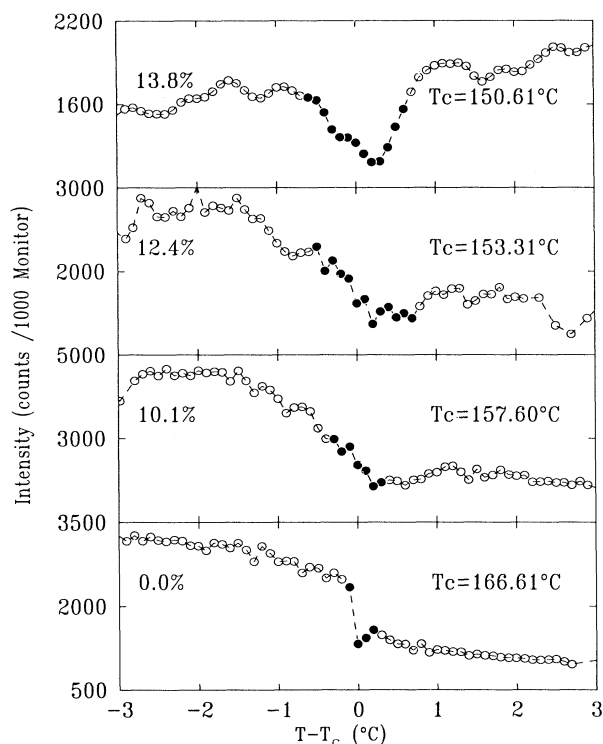
FIG. 16. Temperature dependence of peak intensity of q' reflection, which evolves into the q_0 peak, for 13.8, 12.4, 10.1, and 0.0-mol % 8OCB in the 8OCB-plus-DB7OCN mixtures. The decrease in peak intensity and the associated increase in peak width (Fig. 15) near the Sm- A_d to Sm- A_2 transition are due to the simultaneous presence of the q_0 and q' reflections from the two phases.
