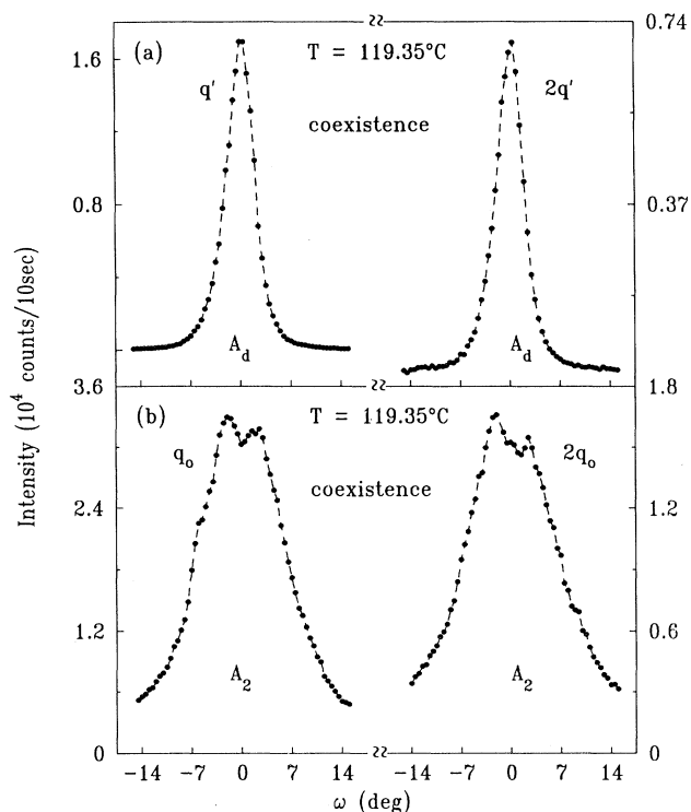
FIG. 10. \omega scans for the 35.1-mol % 8OCB-plus-DB7OCN mixture through (a) the two \text{Sm-A}_d peaks at q'=0.1313 \text{ \AA}^{-1} and 2q'=0.2626 \text{ \AA}^{-1} and (b) the two \text{Sm-A}_2 peaks at q_0=0.1211 \text{ \AA}^{-1} and 2q_0=0.2422 \text{ \AA}^{-1} in the coexistence region, at 119.35^\circ\text{C} .
