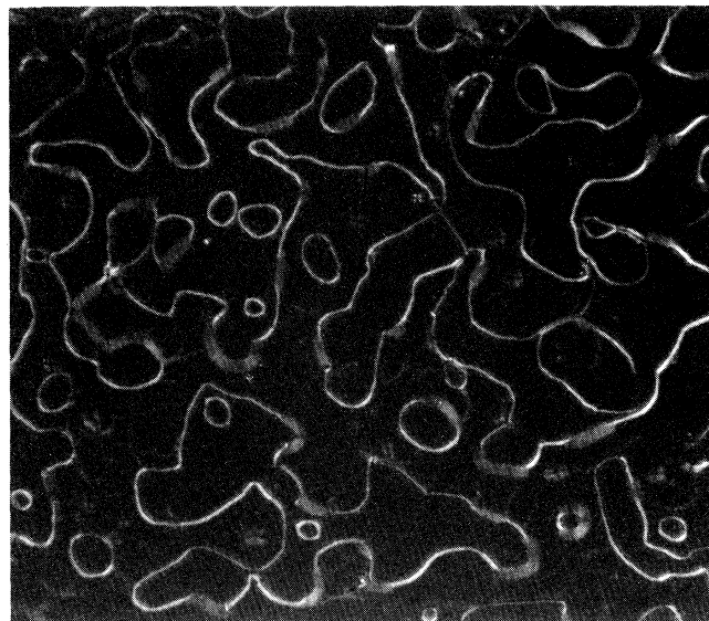
FIG. 14. Upon cooling the homeotropically aligned Sm-A_d phase of the 28.0-mol % mixture into the intermediate region, domains of slightly different contrast separated by bright and relatively sharp lines forming loops are observed. These loops become diffuse with time and disappear upon cooling into the Sm-A_2 phase.
