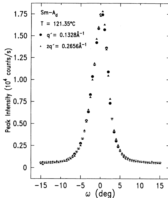
FIG. 9. \omega scans through the two \text{Sm-A}_d peaks shown in Fig. 8 for the 35.1-mol% 8OCB-plus-DB7OCN mixture possess half-widths of \sim 2.3^\circ . The 2q' peak has been scaled by 2.6 and shifted by 375 . The two \omega scans, evidently, are identical.
