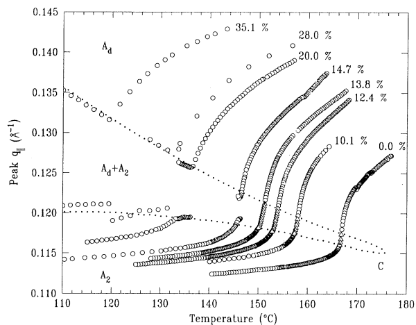
FIG. 7. Temperature dependence of the \text{Sm-A}_d and \text{Sm-A}_2 wave vectors, q' and q_0 , respectively, for eight different concentrations of 8OCB in 8OCB-plus-DB7OCN mixtures. The simultaneous presence of the two peaks over a finite temperature range for concentrations higher than 14 mol % confirms the coexistence of the two phases. At concentrations below 14 mol %, a dramatic increase in peak width and an associated drop in peak intensity are used to infer the coexistence (triangles) as discussed in the text. The dotted line is drawn to approximately represent the outline of the coexistence of the \text{Sm-A}_d and \text{Sm-A}_2 phases.
