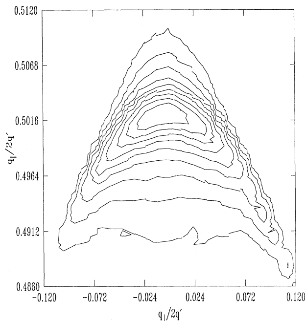
FIG. 13. Equal-intensity contour plots in the q_{\parallel}-q_{\perp} plane in the vicinity of q' reflection in the coexistence region. Contours are drawn at 90, 80, 70, 60, 50, 40, 30, 20, and 10% of peak intensity. These measurements were made at 131.50^\circ\text{C} for the 28.0-mol % 8OCB-plus-DB7OCN mixture. The absence of off-axis peaks rules out the possibility of this region being the Sm-\bar{A} , the Sm-A_{\text{cren}} , or the Sm-\bar{C} phase.
