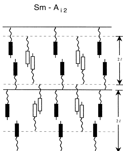
FIG. 5. Real-space representation of the Sm-A_{i2} phase in which Sm-A_d -like (open molecules) and Sm-A_2 -like (dark molecules) molecular arrangements coexist throughout the sample.
