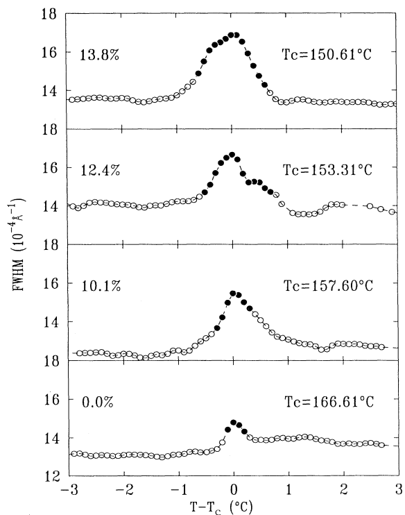
FIG. 15. Temperature dependence of full peak width at half maximum of the q' peak, which evolves into the q_0 peak, for 13.8, 12.4, 10.1, and 0.0-mol % 8OCB in the 8OCB-plus-DB7OCN mixtures. An increase in the peak width near the Sm-A_d to Sm-A_2 transition is due to simultaneous presence of unresolved q' and q_0 peaks from the Sm-A_d and Sm-A_2 phases, respectively.
