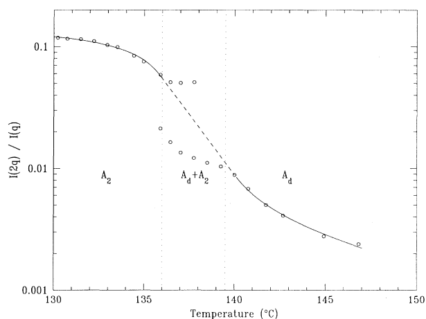
FIG. 12. The ratio of intensities of the second to first reflection in the \text{Sm-A}_d and \text{Sm-A}_2 phases of 280-mol % 8OCB mixture. This ratio increases with decreasing temperature and qualitatively represents the relative growth of the order parameter \psi_2 at the \text{Sm-A}_d to \text{Sm-A}_2 transition. Wide coexistence at this phase transition is evident. Lines through the data points are drawn as a guide to the eye.
