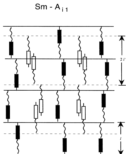
FIG. 4. Real-space representation of the incommensurate Sm-A_{i1} phase. Two interpenetrating smectic modulations with periodicities of l (dark molecules) and 2l' (open molecules, with overlapping dimerlike arrangements) coexist in the Sm-A_{i1} phase.
