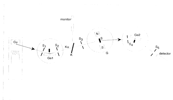
FIG. 6. Schematic representation of the high-resolution x-ray-diffraction experiment. Here, Cu represents the copper target of the Rigaku rotating anode source, and Ge1 and Ge2 are single germanium crystals used as the monochromator to select K\alpha radiation and the analyzer, respectively. G is a two-circle Huber goniometer with angular precision of 0.00025^\circ for \theta and 2\theta motions, S_1 , S_2 , S_3 , S_4 , and S_5 are collimating slits, S is the sample in the magnetic field produced by a pair of rare-earth permanent magnets N and S , and K represents a thin Kapton sheet used to scatter a small fraction of the beam into the monitor.
