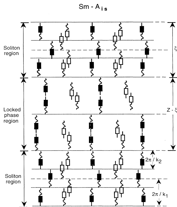
FIG. 3. Real-space representation of the incommensurate soliton \text{Sm-}A_{is} phase. The central rigid part of molecules is represented by the rectangle, aliphatic tail by wavy lines, and the dipoles by a short straight line on one side of the rectangle. In this phase, regions of width \xi with two independent wave vectors k_1 and k_2 separate regions of width Z-\xi in which the two modulations are phase locked. The molecules form dimerlike arrangements with no overlap (filled rectangles) or with some lengthwise overlap (unfilled rectangles).
